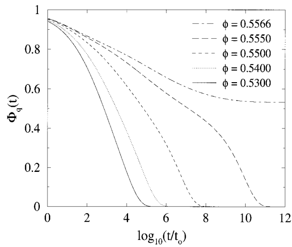
FIG. 3. Density correlator for q\sigma=14.4 at \tau=1.40 and various \phi as a function of \log_{10}(t/t_0) with t_0=\sigma/v .
